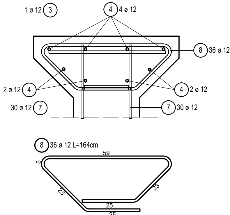
Detail 1 M1:10
